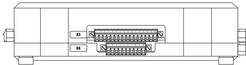
View "A"
